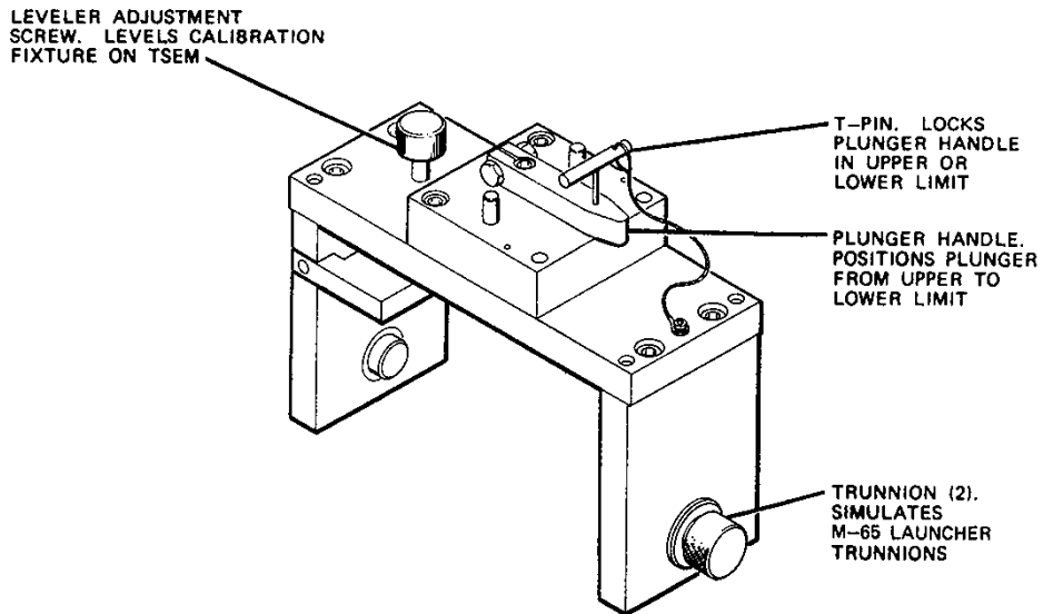
TSEM SHEAR PIN CALIBRATION TESTER
