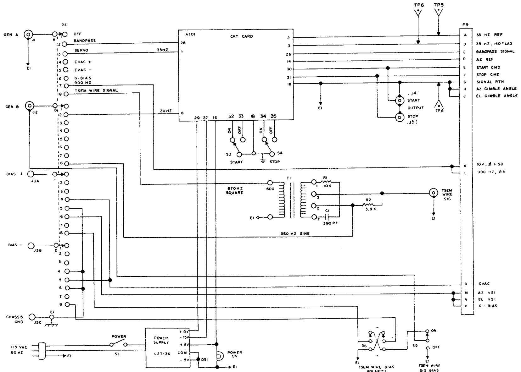
Calibration control schematic.
